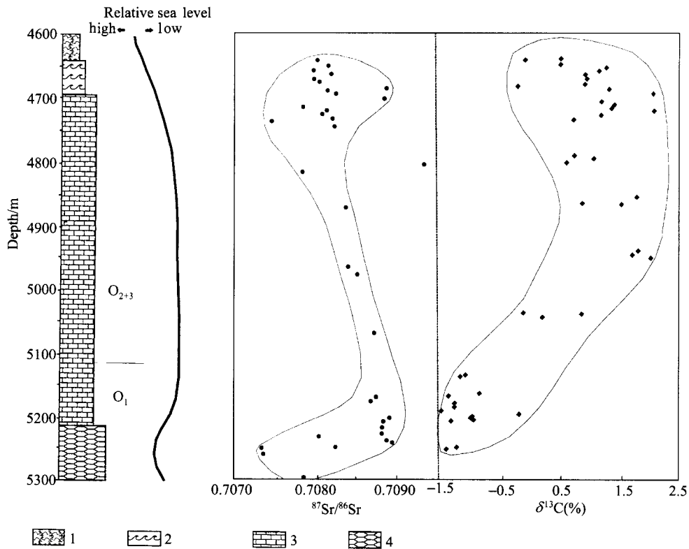
Fig. 1. The relationships between sea-level fluctuations and \delta^{13}\text{C} , ^{87}\text{Sr}/^{86}\text{Sr} values in the Ordovician of well Tazhong 12. 1, Mixed shelf facies; 2, shelf storm sedimentary facies; 3, open platform facies; 4, restricted platform facies.
