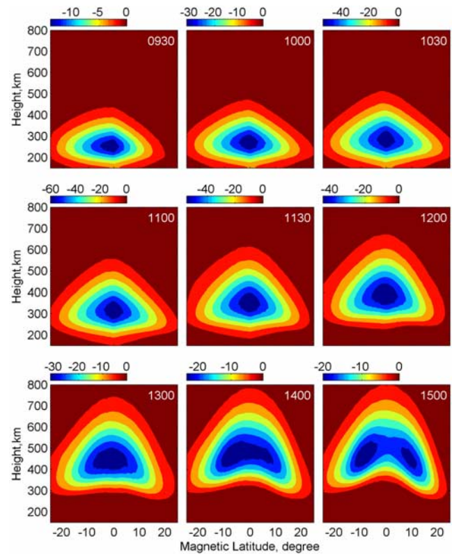
Figure 8. The evolutions of absolute change in Ne (in unit of 10^{10} \text{el}/\text{m}^3 ) from 0930 LT to 1500 LT when a solar eclipse occurred at the magnetic equator. The text in each panel indicates the local time.
