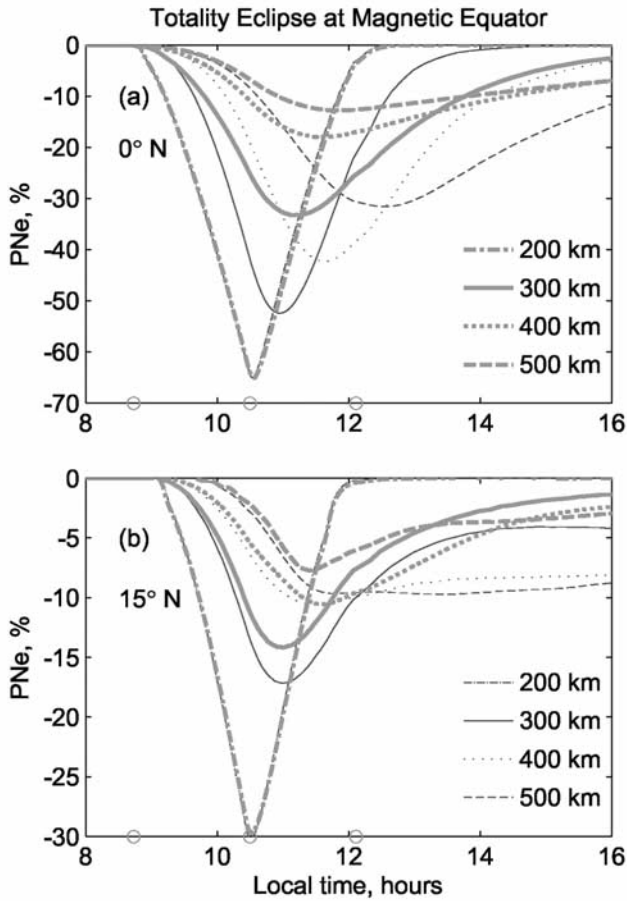
Figure 7. Temporal variation of the PNe at various height at (a) magnetic equator (0°N) and (b) EIA region (15°N) when a total eclipse occurred at the equator. The bold lines indicate the results with E \times B drift considered, and the thin lines indicate the results with E \times B not considered. The circles in the x axis indicate the beginning, totality, and end of the eclipse.
