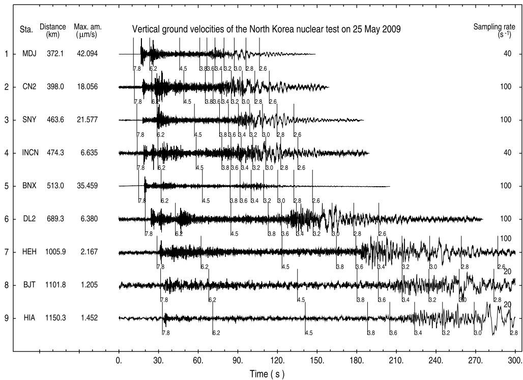
Figure 2. Vertical ground velocities observed from the 25 May 2009 North Korean nuclear explosion. The traces are ordered according to their epicentral distances. The station names and peak amplitudes in \mu\text{m/s} are listed on the left side, and the corresponding sampling rates are listed on the right side. The vertical bars and numbers on the traces indicate apparent group velocities.
