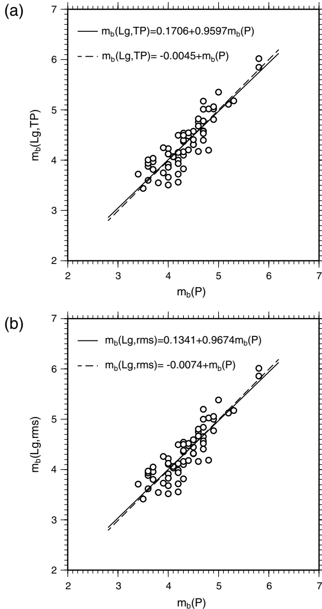
Figure 4. Comparisons between the global body-wave magnitudes and the regional Lg -wave magnitudes for all 82 regional events listed in Table S1 (available in the electric supplement to this paper) with (a) m_b(Lg, TP) versus m_b(P) and (b) m_b(Lg, rms) versus m_b(P) . The solid lines are from least squares fittings and the dashed lines are for a fixed unit slope.
