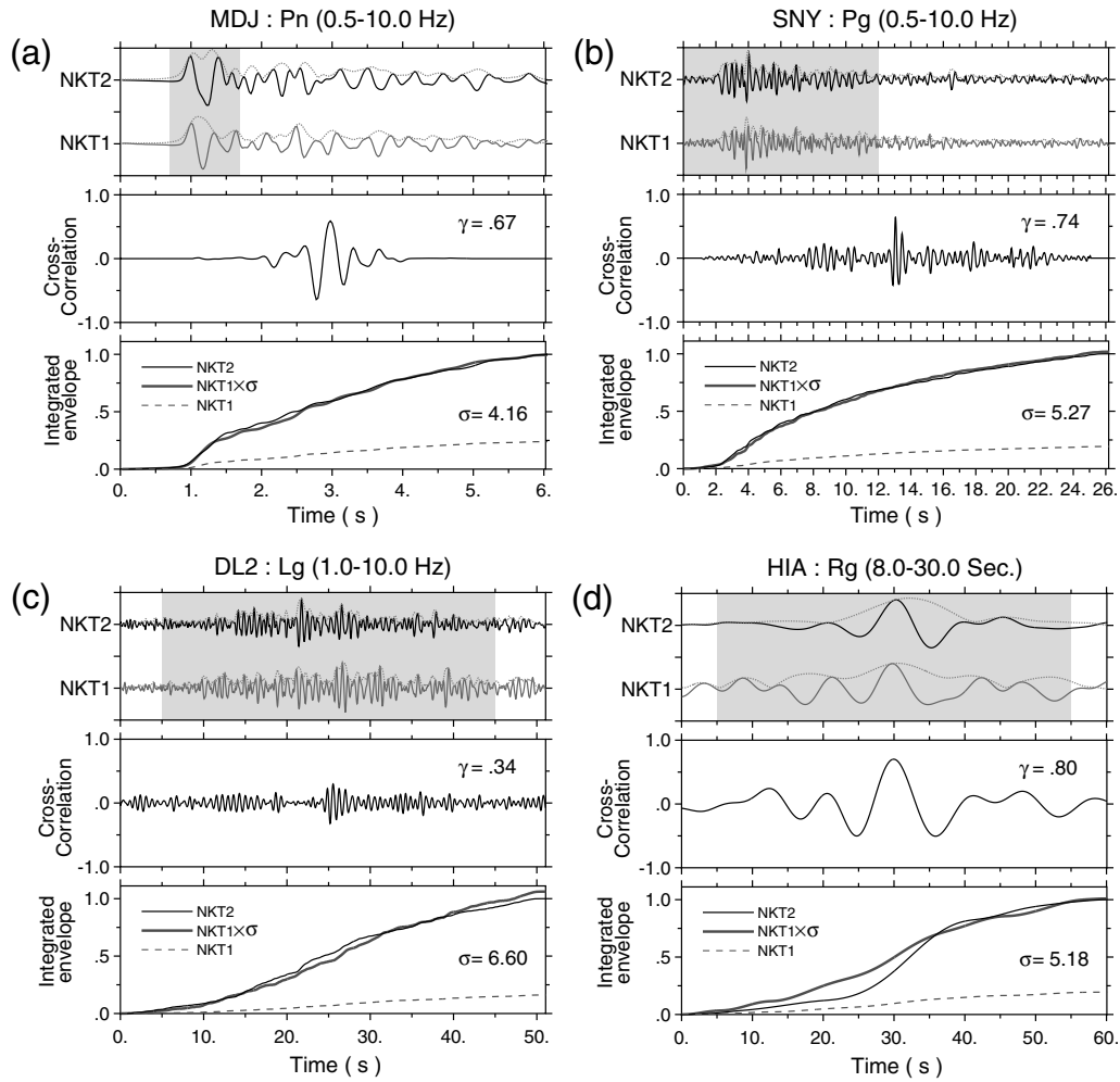
Figure 3. Comparison between regional waveforms from the two North Korean nuclear tests at selected stations. For each station, band-pass-filtered waveforms and their envelopes are shown in the upper panel. Shown in the middle panels is the cross-correlation function. Illustrated in the lower panel are integrated amplitude envelopes. Note that the curve from NKT1 has been multiplied by a factor to match that from NKT2. The maximum correlation coefficients \gamma and the ratio \sigma between the integrated envelopes are labeled in the figure.
